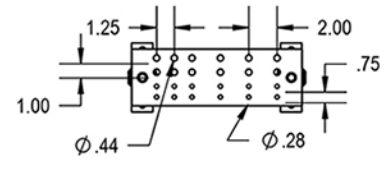
SCGB-6 - 4" x 12" 24 Holes w/6 Taps
