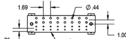
SCGB-8 - 4" x 16" 34 Holes w/34 Taps
