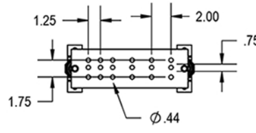
SCGB-5 - 4" x 12" w/18 Holes
